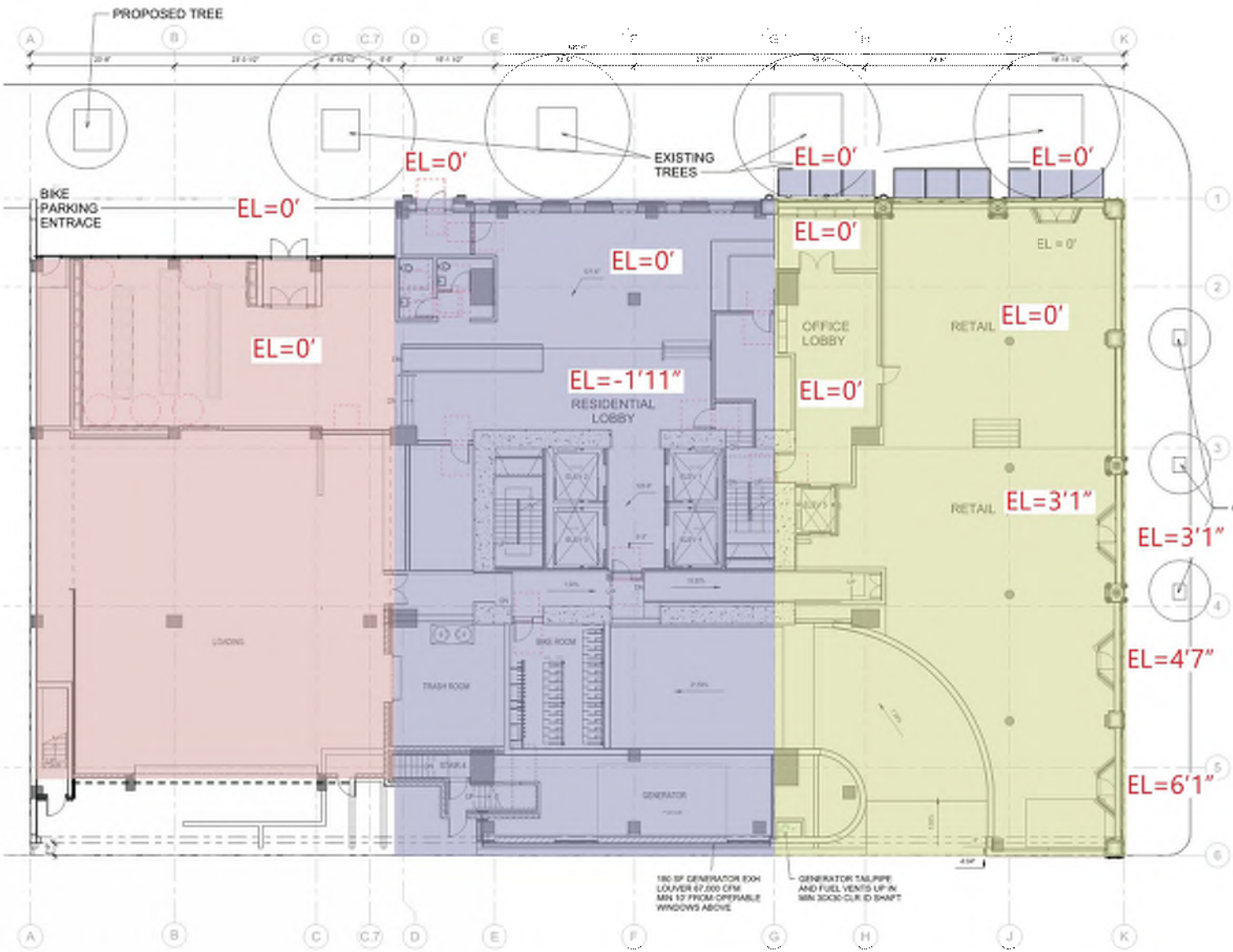
NEW L1 PLAN
